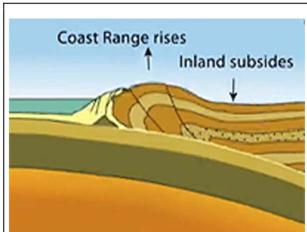
VIDEO: This animation illustrates how the subduction of an oceanic plate can eventually trigger a great earthquake and tsunami.
