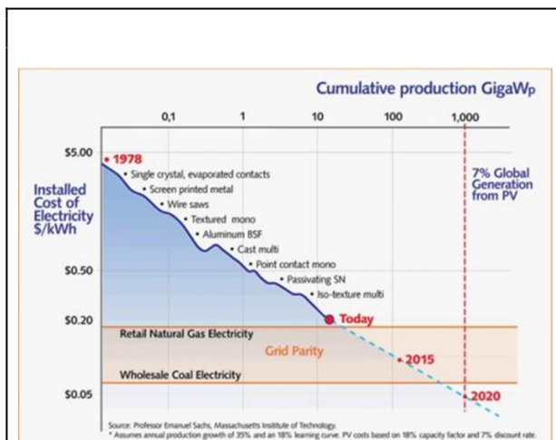
Projected photovoltaic energy costs
