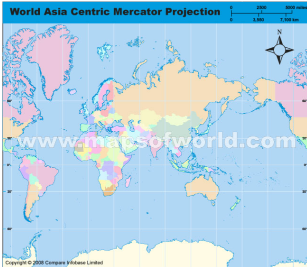
An Asia-centered Mercator projection of the world
