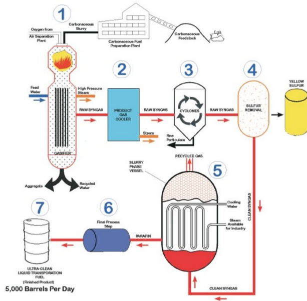
Coal liquefaction process
