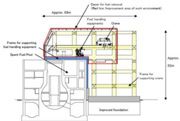
Fig.2 Schematic Diagram of the Cover for Fuel Removal
